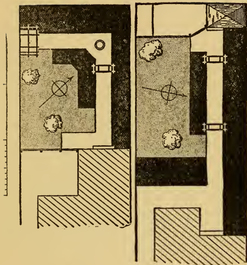
Fig. 69. —Size, 26 feet by 20 feet. Aspect, SE. The path at its near end communicates with the kitchen yard, and at its far end terminates at an arbour. The space at the angle of the path might carry a tub or sundial. The north-west boundary fence might be raised with trellis to give increased surface for growing climbing plants.
